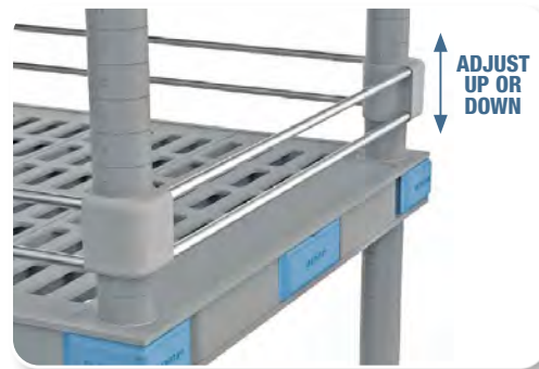
ADJUSTABLE HEIGHT SIDE AND BACK LEDGE QPL 2-1/4" Height
