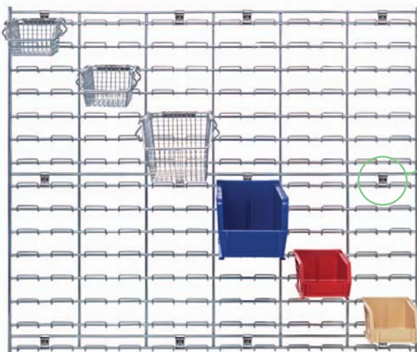
WLP-3036C 36"L x 30"H Accepts all sizes of Ultra Stack & Hang Bins and Mesh Bins. Includes 12 direct mount clips. 175 lb. load capacity. (Bins sold separately)
