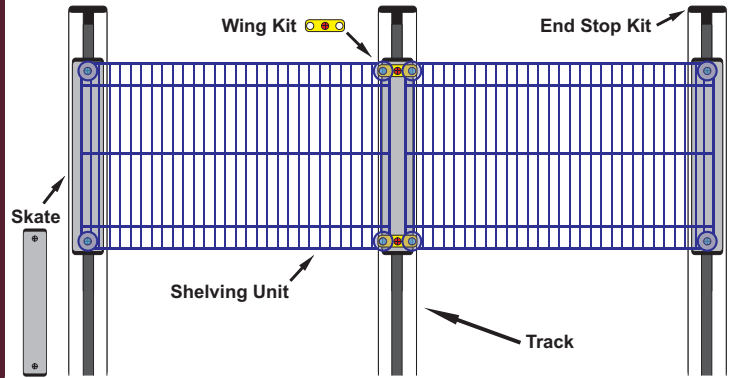
DOUBLE UNIT TRACK SYSTEM (Top View)
